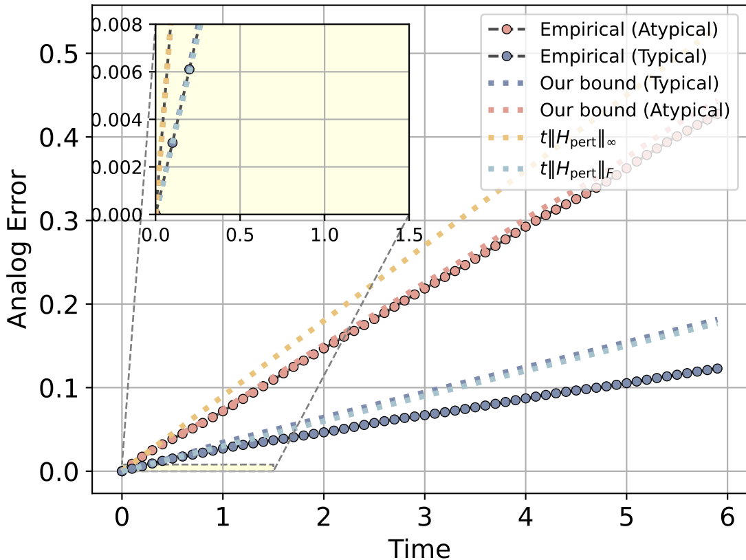
TFIM, long-time evolution with imperfections
